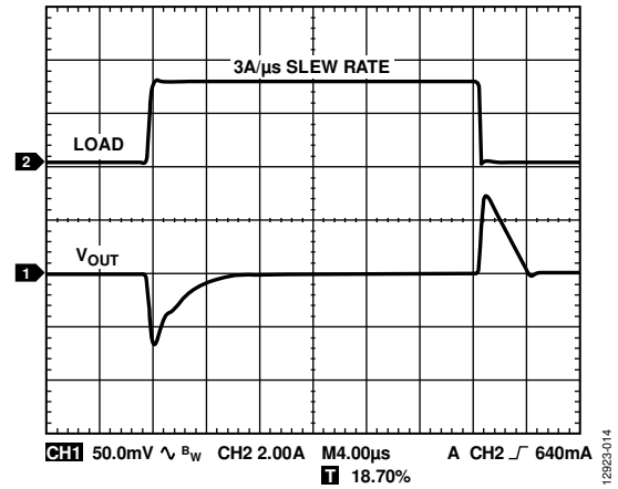
Figure 14. Load Transient Response, C_{OUT} = 10\ \mu\text{F} , V_{IN} = 1.8\text{ V} , V_{OUT} = 1.3\text{ V}
