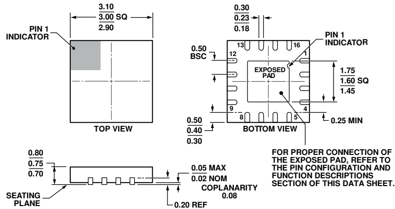
Figure 49. 16-Lead Lead Frame Chip Scale Package [LFCS] 3 mm × 3 mm Body and 0.75 mm Package Height (CP-16-22) Dimensions shown in millimeters
