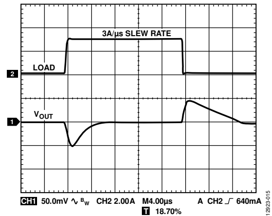
Figure 15. Load Transient Response, C_{OUT} = 47\ \mu\text{F} , V_{IN} = 1.8\text{ V} , V_{OUT} = 1.3\text{ V}
