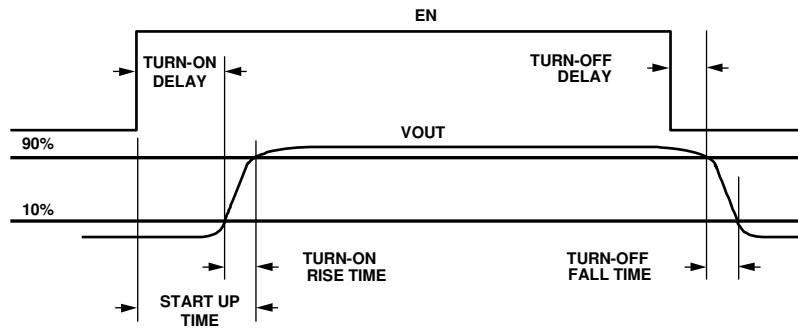
Figure 3. Timing Diagram
