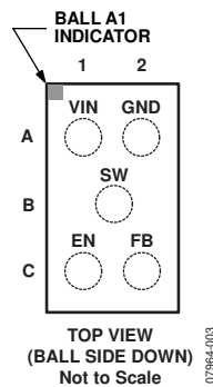
Figure 2. Pin Configuration
