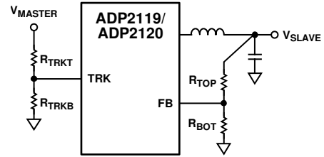
Figure 51. Voltage Tracking
