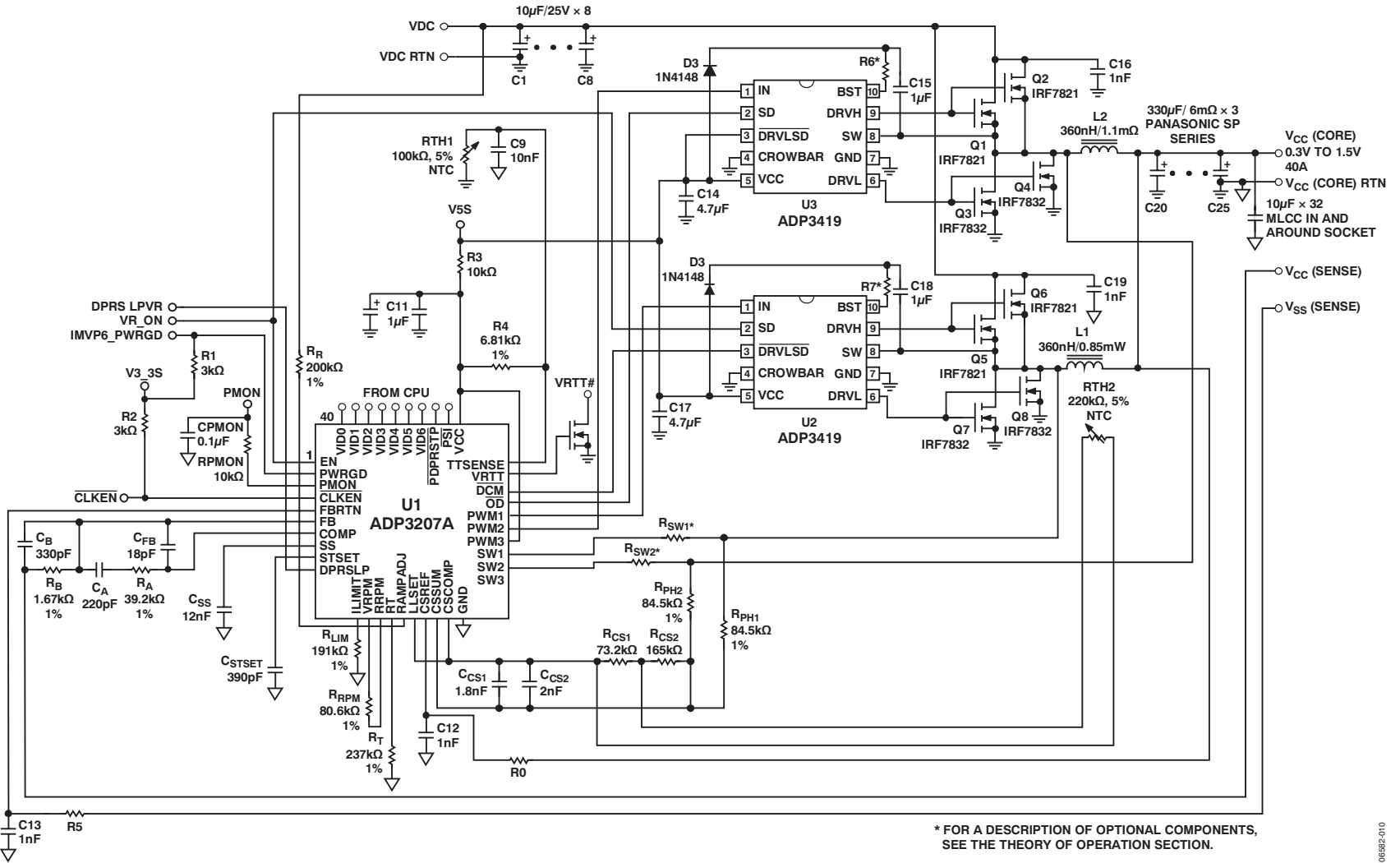
Figure 11. Typical 2-Phase Application Circuit
