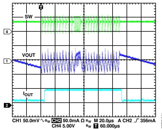
Figure 26. BUCK1 Response to Load Transient, I_{OUT1} from 1\text{ mA} to 50\text{ mA} , V_{OUT1} = 3.3\text{ V} , Auto Mode
