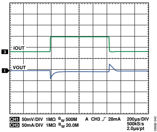
Figure 35. LDO Response to Load Transient, I_{OUT2} from 1\text{ mA} to 80\text{ mA} , V_{OUT2} = 3.3\text{ V}
