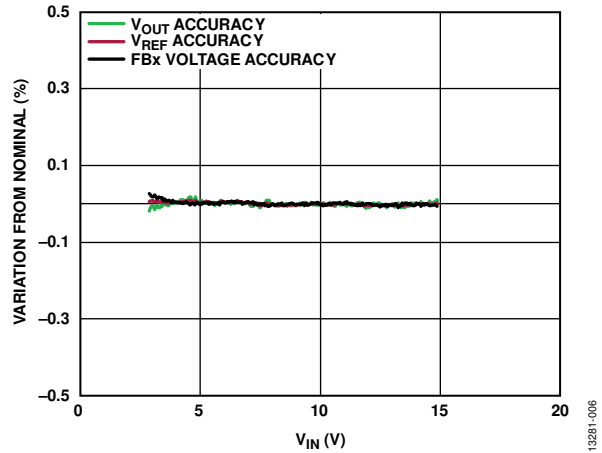
Figure 6. Inverting Regulator Line Regulation, V_{NEG} = -15\text{ V} , f_{SW} = 1.2\text{ MHz} , 15 mA Load, T_A = 25^\circ\text{C} (Nominal Defined as Average Value Within a Range of 10% to 90% V_{IN} )
