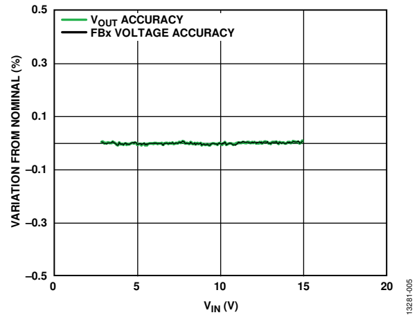
Figure 5. Boost Regulator Line Regulation, V_{POS} = 15\text{ V} , f_{SW} = 1.2\text{ MHz} , 15 mA Load, T_A = 25^\circ\text{C} (Nominal Defined as Average Value Within a Range of 10% to 90% V_{IN} )
