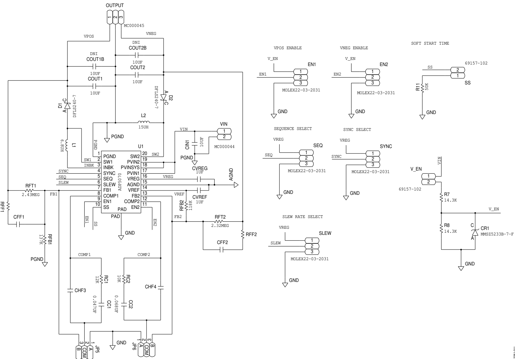
Figure 11. Evaluation Board Schematic for the ADP5070/ADP5071 Rev. 0 | Page 8 of 13
