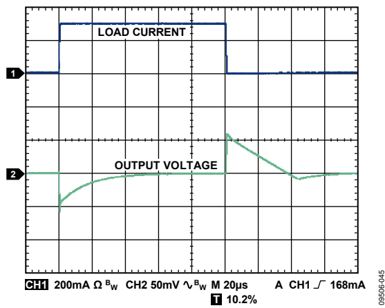
Figure 52. Load Transient Response, C_{IN}, C_{OUT} = 1 \mu F , I_{LOAD} = 1 mA to 300 mA , V_{OUT} = 3.3 V , V_{IN} = 5 V
