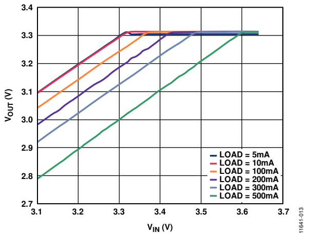
Figure 13. Output Voltage vs. Input Voltage (in Dropout), V_{OUT} = 3.3 V
