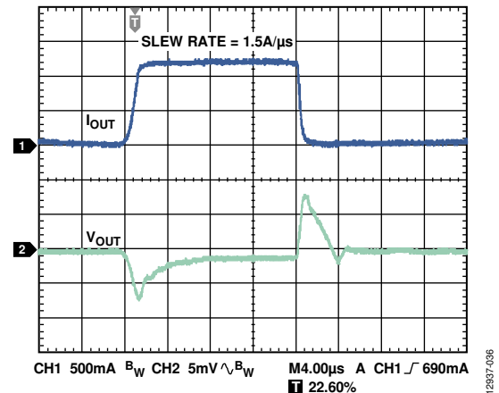
Figure 34. Load Transient Response, I_{LOAD} = 100\text{ mA} to 1.2\text{ A} , V_{OUT} = 3.3\text{ V} , V_{IN} = 4.0\text{ V} , C_{OUT} = 22\text{ }\mu\text{F} , Channel 1 = I_{OUT} , Channel 2 = V_{OUT}
