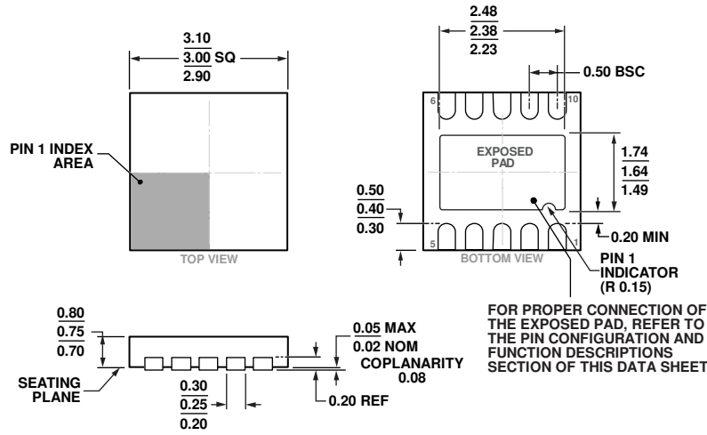
Figure 64. 10-Lead Lead Frame Chip Scale Package [LFCS] 3 mm x 3 mm Body and 0.75 mm Package Height (CP-10-9) Dimensions shown in millimeters
