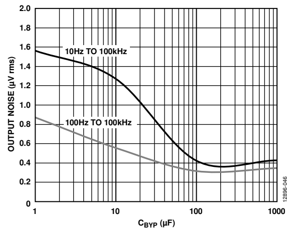
Figure 44. RMS Noise vs. Bypass Capacitance ( C_{BYP} )
