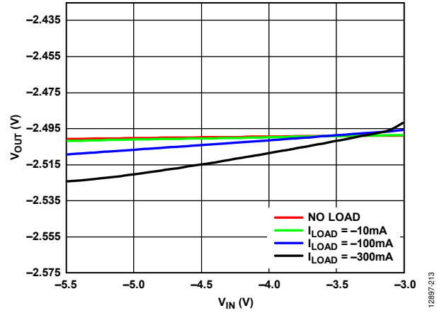
Figure 13. Output Voltage ( V_{OUT} ) vs. Input Voltage ( V_{IN} ), V_{OUT} = -2.5 V
