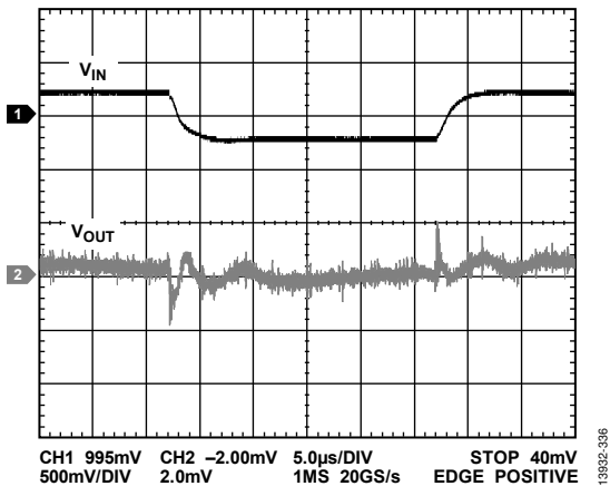
Figure 36. Line Transient Response, 500 mV Step, V_{OUT} = -1.2V , I_{LOAD} = -500mA
