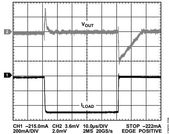
Figure 39. Load Transient Response, V_{OUT} = -2.5V , I_{LOAD} = -10mA to -500mA
