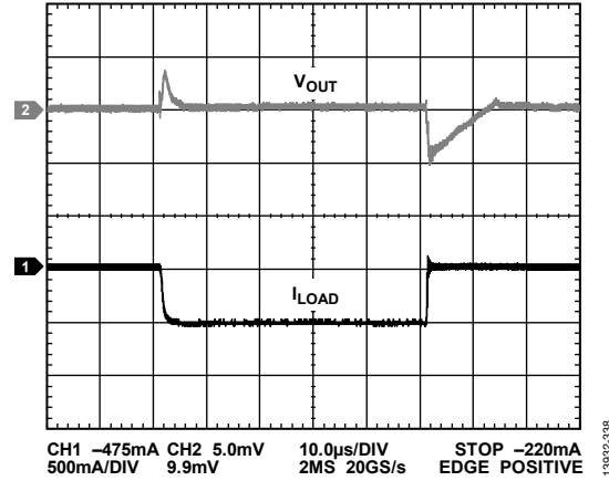
Figure 38. Load Transient Response, V_{OUT} = -1.2V , I_{LOAD} = -10mA to -500mA
