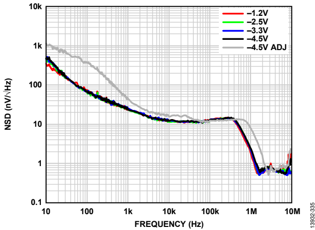
Figure 35. Noise Spectral Density (NSD) vs. Frequency at Various Output Voltages, V_{IN} = -3.8V , V_{OUT} = -3.3V
