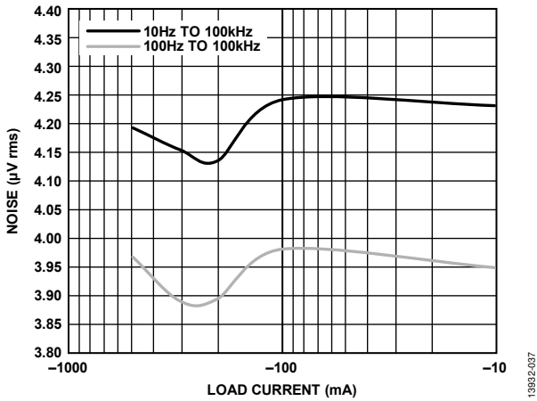
Figure 34. RMS Noise vs. Load Current ( I_{LOAD} ) at Various Frequencies, V_{IN} = -3.8V , V_{OUT} = -3.3V
