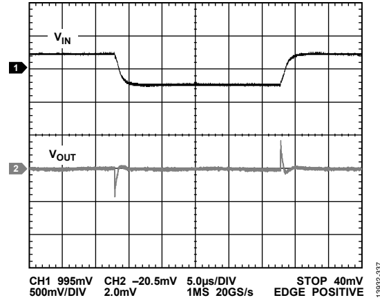
Figure 37. Line Transient Response, 500 mV Step, V_{OUT} = -3.3V , I_{LOAD} = -500mA
