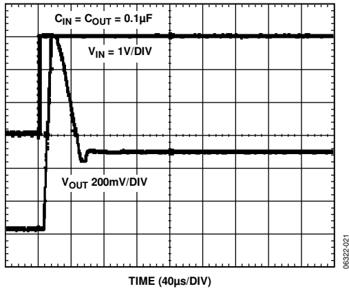
Figure 21. Turn-On Response, V_{OUT} = 0.5\text{ V}
