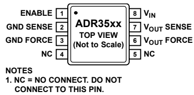
Figure 2. Pin Configuration
