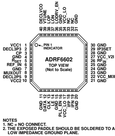
Figure 3. Pin Configuration
