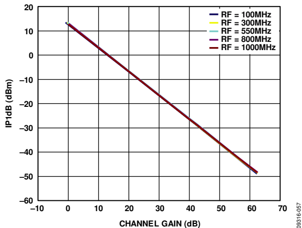
Figure 11. Input 1dB Compression Point (IP1dB) vs. Channel Gain, and RF Input Frequency, V_{OCM} = 1.6V , Nominal Conditions, Narrow-Band Mode
