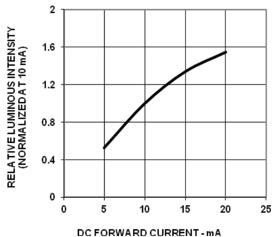
Fig 1: Relative Luminous Intensity Vs Forward Current
