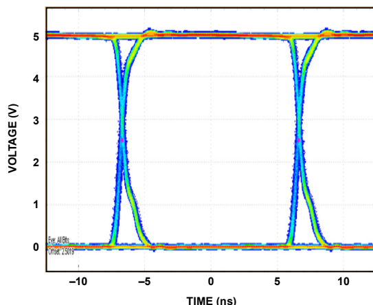
Figure 21. Eye Diagram
