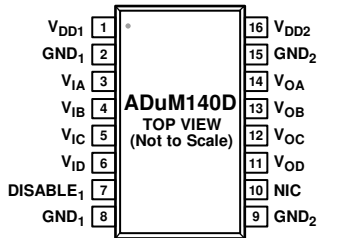
Figure 7. ADuM140D Pin Configuration
