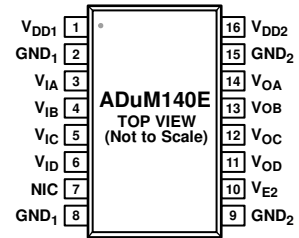
Figure 8. ADuM140E Pin Configuration
