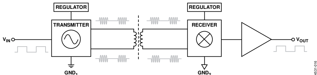
Figure 16. Operational Block Diagram of a Single Channel with a Low Fail-Safe Output State
