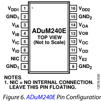
Figure 6. ADuM240E Pin Configuration
