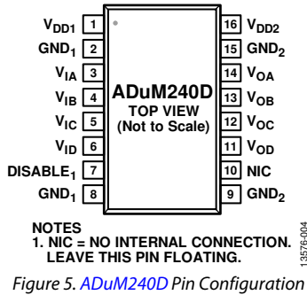
Figure 5. ADuM240D Pin Configuration
