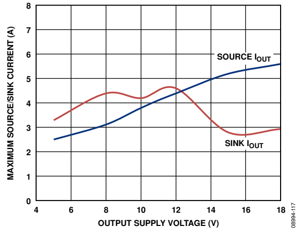
Figure 18. Typical Maximum Source/Sink Current vs. Output Supply Voltage
