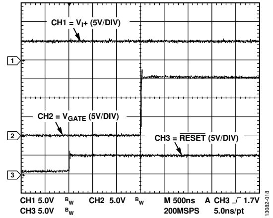
Figure 18. Example \overline{RESET} to Output Valid
