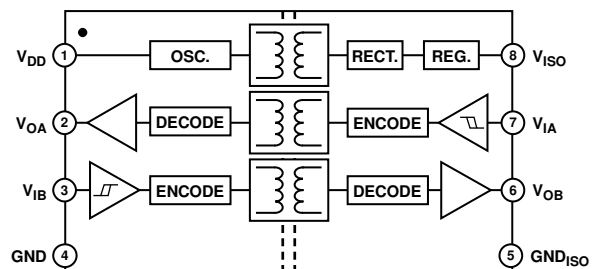
Figure 2. ADuM5241
