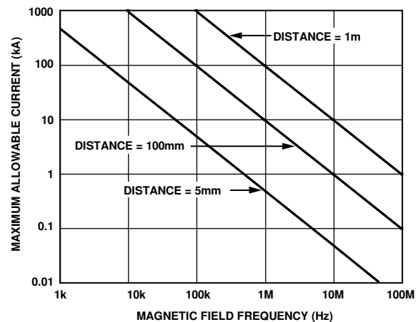
Figure 20. Maximum Allowable Current for Various Current-to-ADuM6132 Spacings
