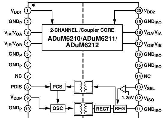
Figure 1. ADuM6210/ADuM6211/ADuM6212
