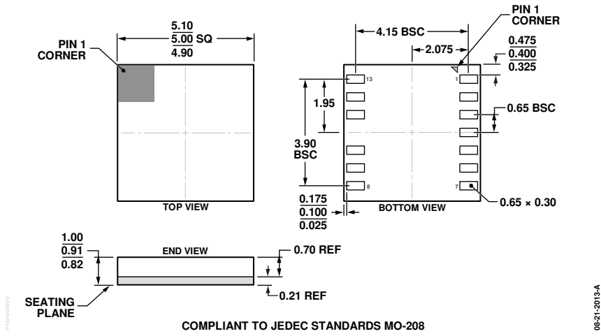
Figure 23. 13-Terminal Land Grid Array [LGA] (CC-13-1) Dimensions shown in millimeters
