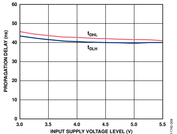
Figure 9. Typical Propagation Delay vs. Input Supply Voltage, V_{DD1}/V_{DD2} = 12 V
