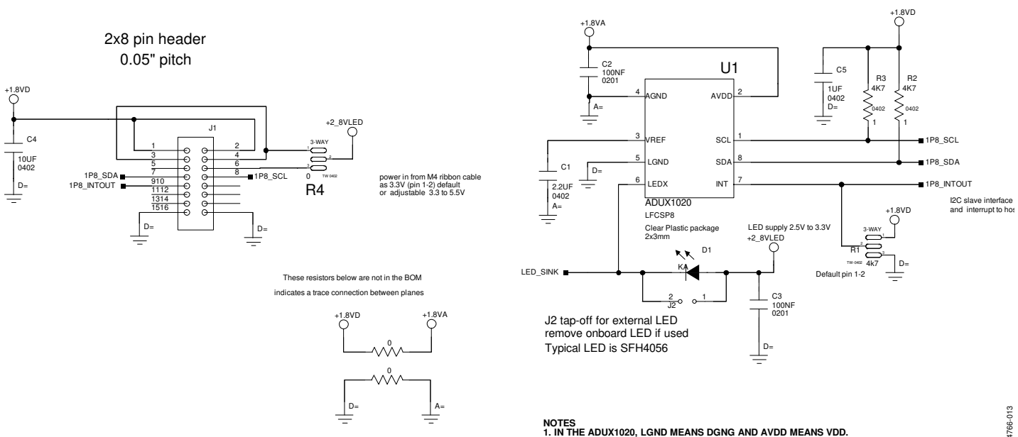
Figure 13. ADUX1020-EVAL-SMALL Small Form-Factor Breakout Board Schematic
