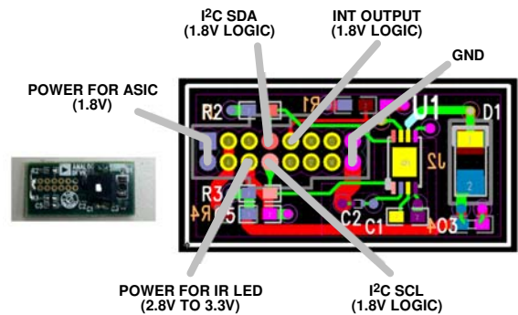
Figure 11. ADUX1020-EVAL-SMALL Breakout Board
