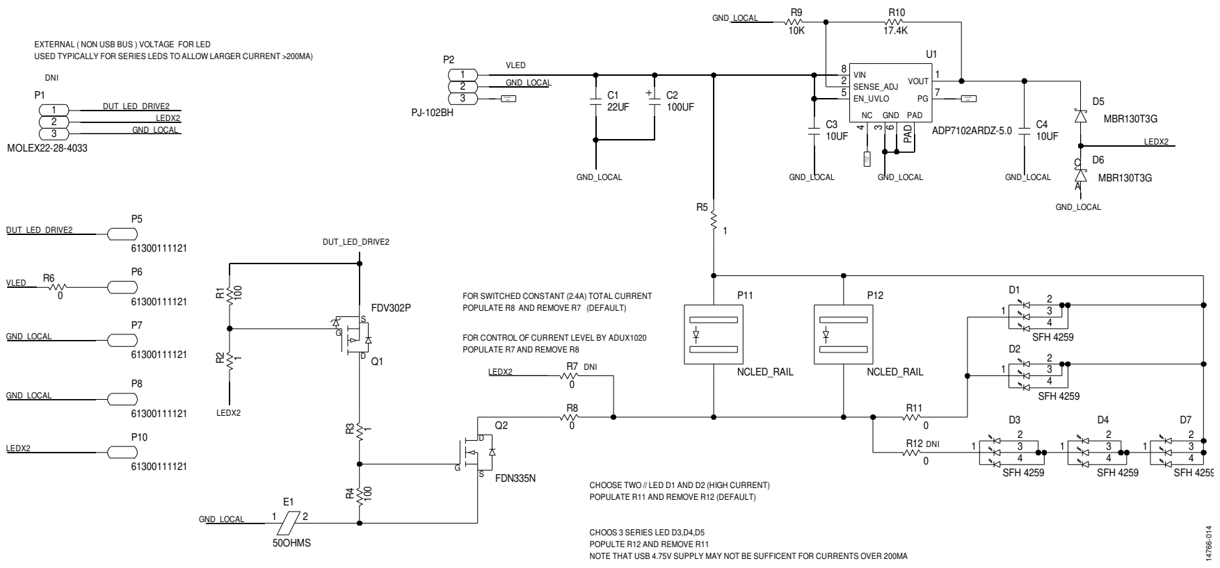
Figure 14. ADUX1020-EVALZ-LED High power LED daughterboard Schematic Rev. 0 | Page 8 of 9
