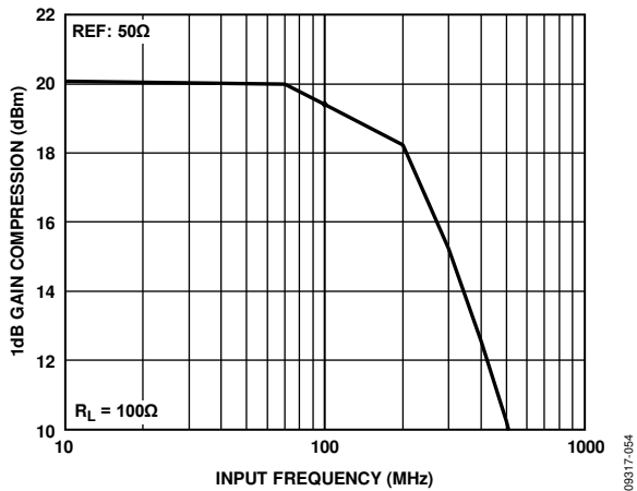
Figure 51. ADV3225 1 dB Gain Compression, 100 Ω Load
