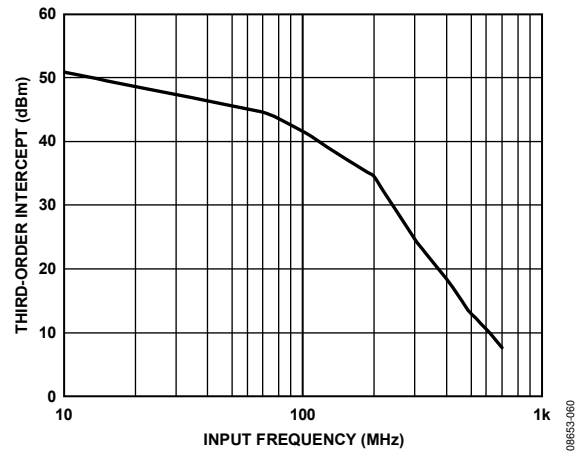
Figure 54. ADV3227 Third-Order Intercept, 100 Ω Load
