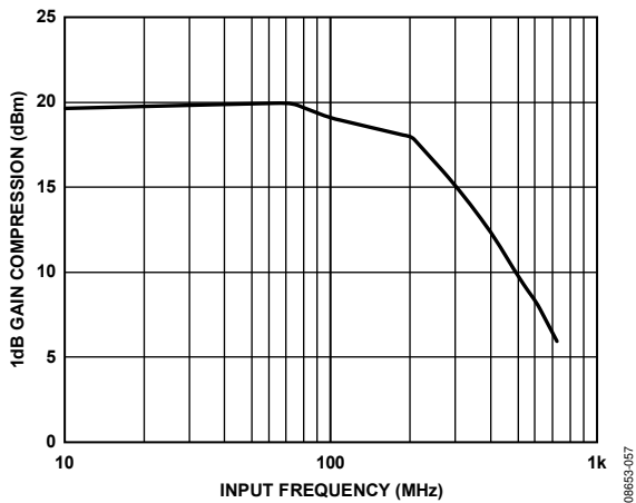
Figure 51. ADV3227 1 dB Gain Compression, 100 Ω Load
