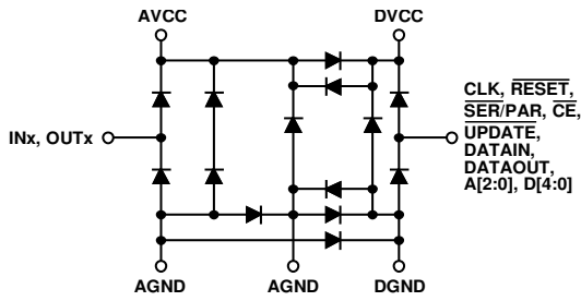
Figure 60. ESD Map
