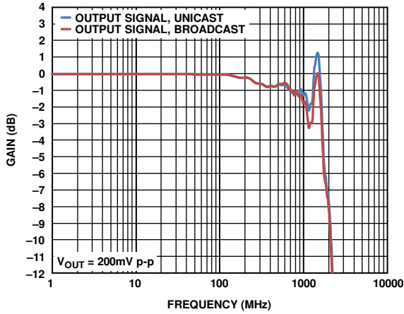
Figure 7. ADV3228 Small Signal Frequency Response
