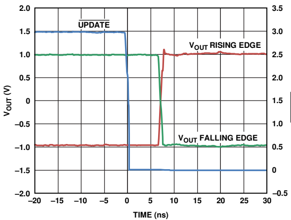
Figure 39. ADV3228 Switching Time
