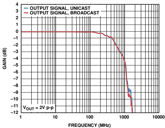
Figure 8. ADV3228 Large Signal Frequency Response
