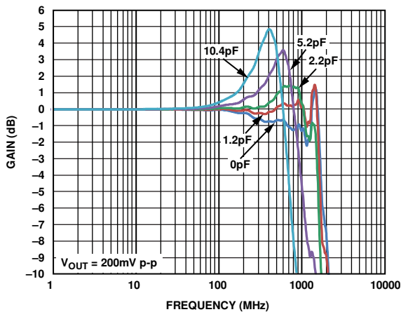
Figure 9. ADV3228 Small Signal Frequency Response with Capacitive Loads
