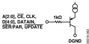
Figure 61. Logic Input
