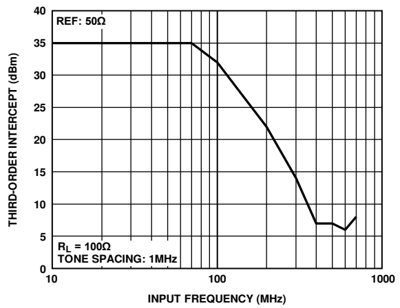
Figure 54. ADV3229 Third-Order Intercept, 100 \Omega Load
