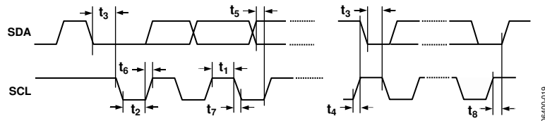
Figure 19. MPU Port Timing Diagram (I 2 C Mode)
