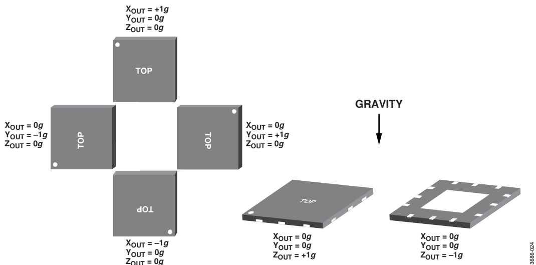
Figure 23. Output Response vs. Orientation to Gravity
