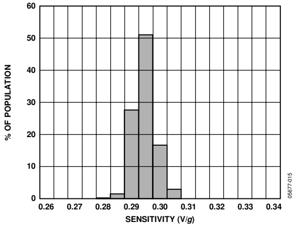
Figure 17. X-Axis Sensitivity at 25°C, V_S = 3 V
