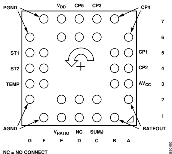
Figure 3. Pin Configuration
