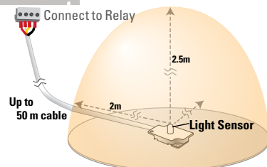
180° 2-meter Half-Sphere Sensor Viewing Angle
