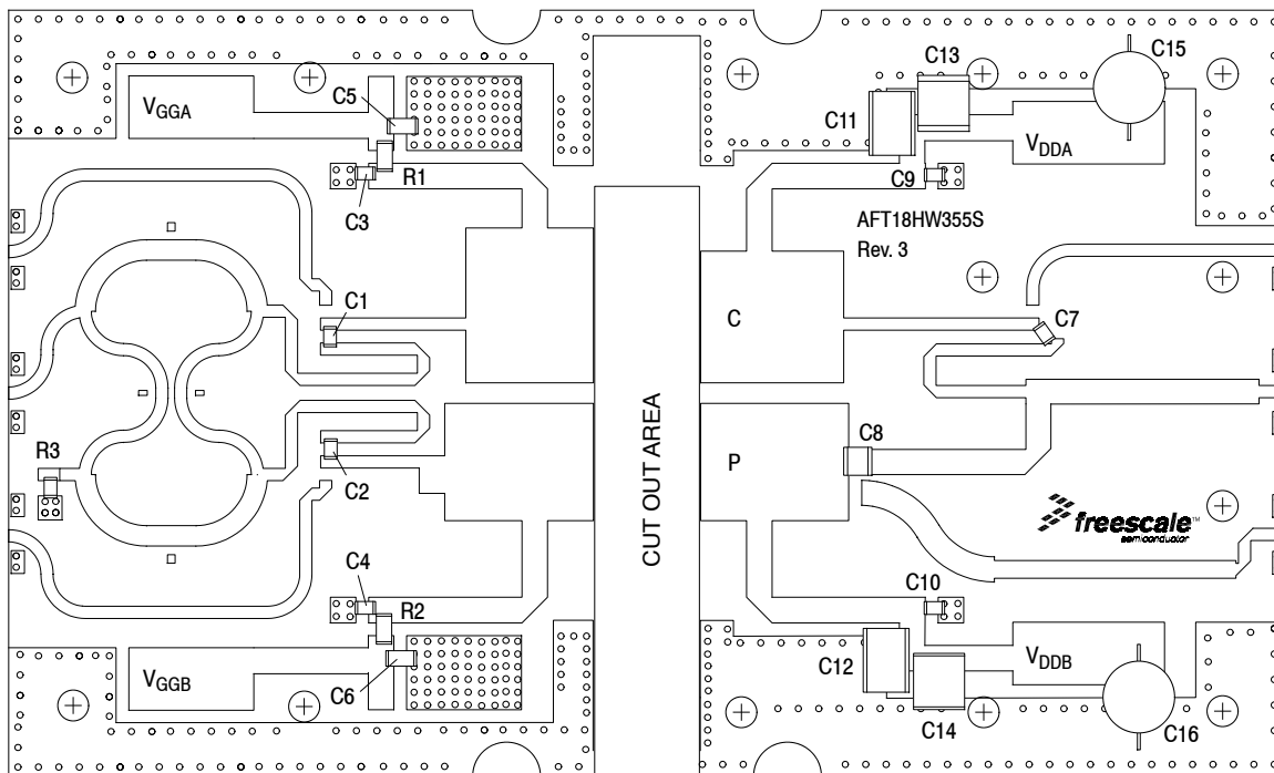
Figure 2. AFT18HW355SR6 Test Circuit Component Layout
