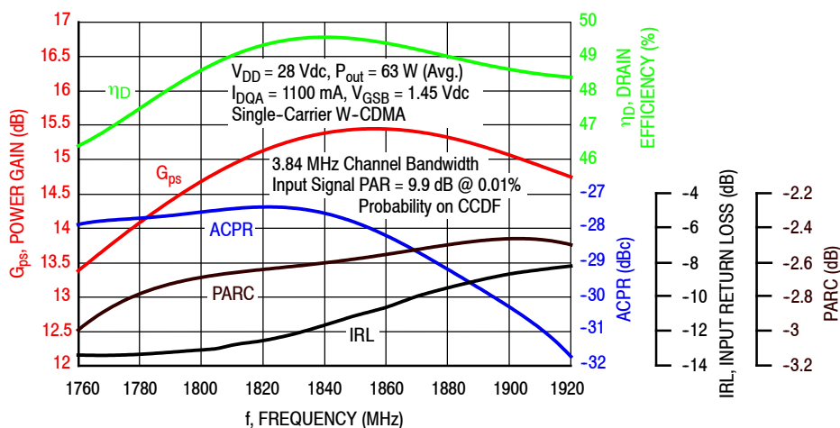
Figure 3. Single-Carrier Output Peak-to-Average Ratio Compression (PARC) Broadband Performance @ P_{out} = 63 Watts Avg.
