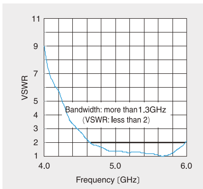
VSWR特性の代表例 (104N 5GHz帯) Typical characteristics of VSWR (104N 5GHz band)
