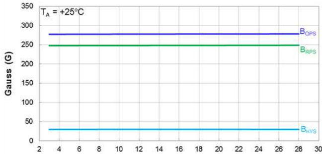
Switch Points B_{OPS} and B_{RPS} vs Supply Voltage
