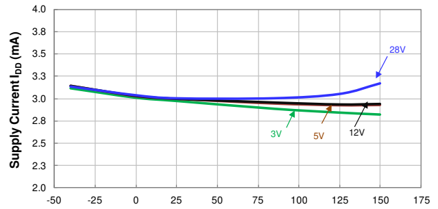
Temperature (°C) Supply Current vs Temperature
