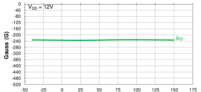
Temperature (°C) Switch Release Points Brp vs Temperature
