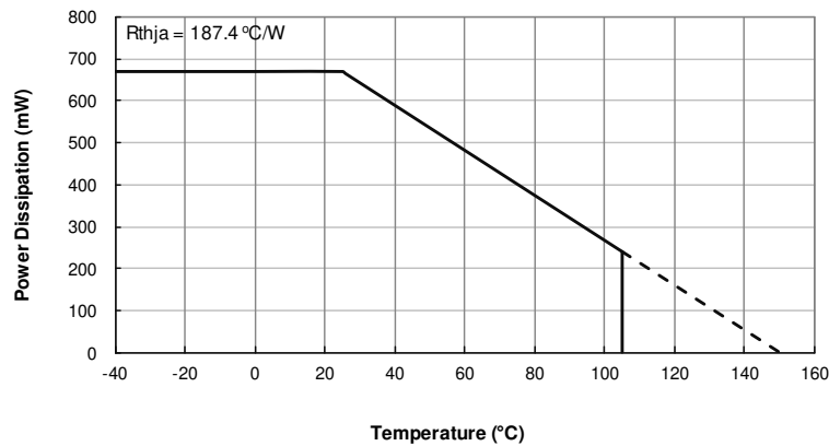
U-DFN2020-6 Thermal Derating Curve
