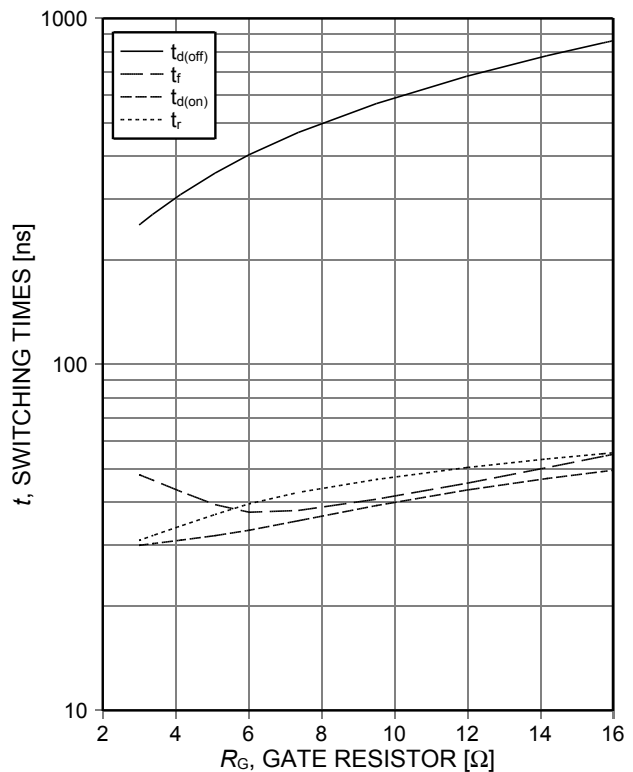
Figure 8. Typical switching times as a function of gate resistor (inductive load, T vj =175°C, V CE =400V, V GE =0/15V, I C =75A, Dynamic test circuit in Figure E)
