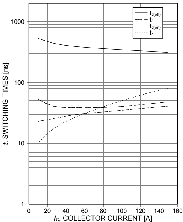
Figure 7. Typical switching times as a function of collector current (inductive load, T vj =175°C, V CE =400V, V GE =0/15V, R G =5Ω, Dynamic test circuit in Figure E)
