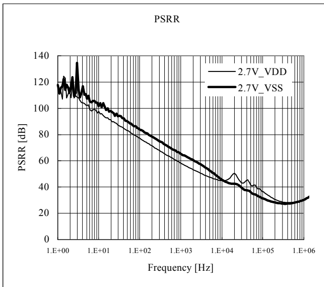
□ Power Supply Rejection Ratio vs. Frequency (VDD=2.7V, Ta=25°C)
