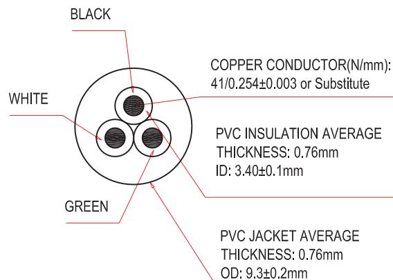
Wire cross section
