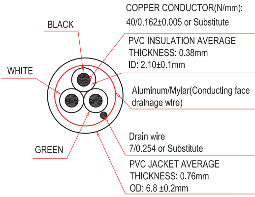
Wire Cross Section
