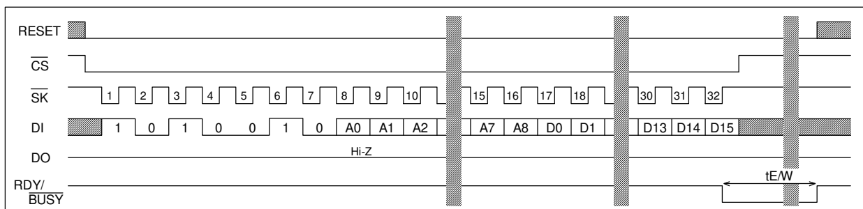
WRITE (AK6481C)
