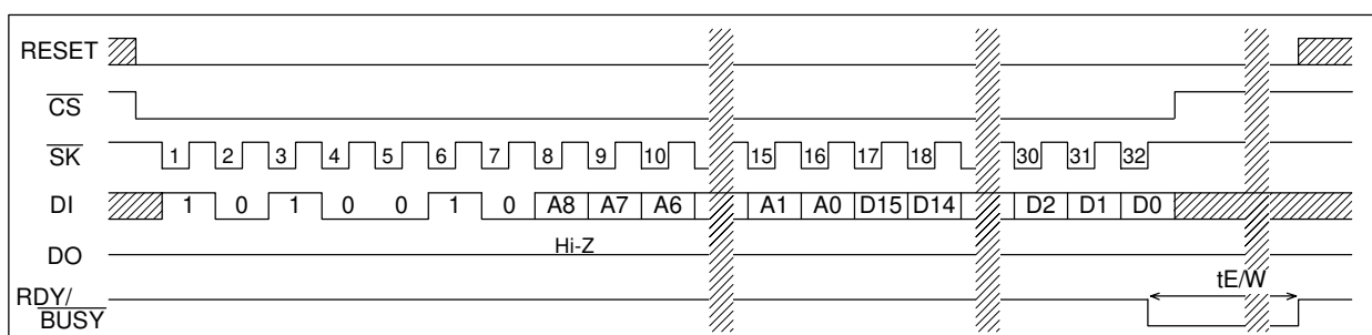
WRITE (AK6480C)
