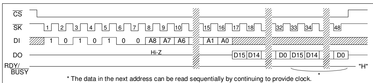
READ (AK6480C)
