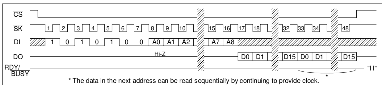
READ (AK6481C)
