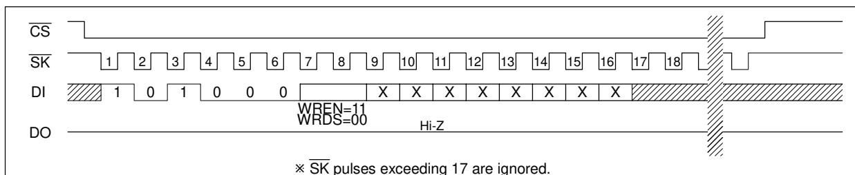
WREN / WRDS
