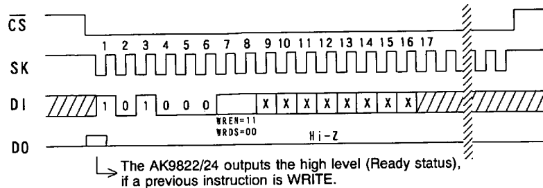
WREN/WRDS (AK9822/24)
